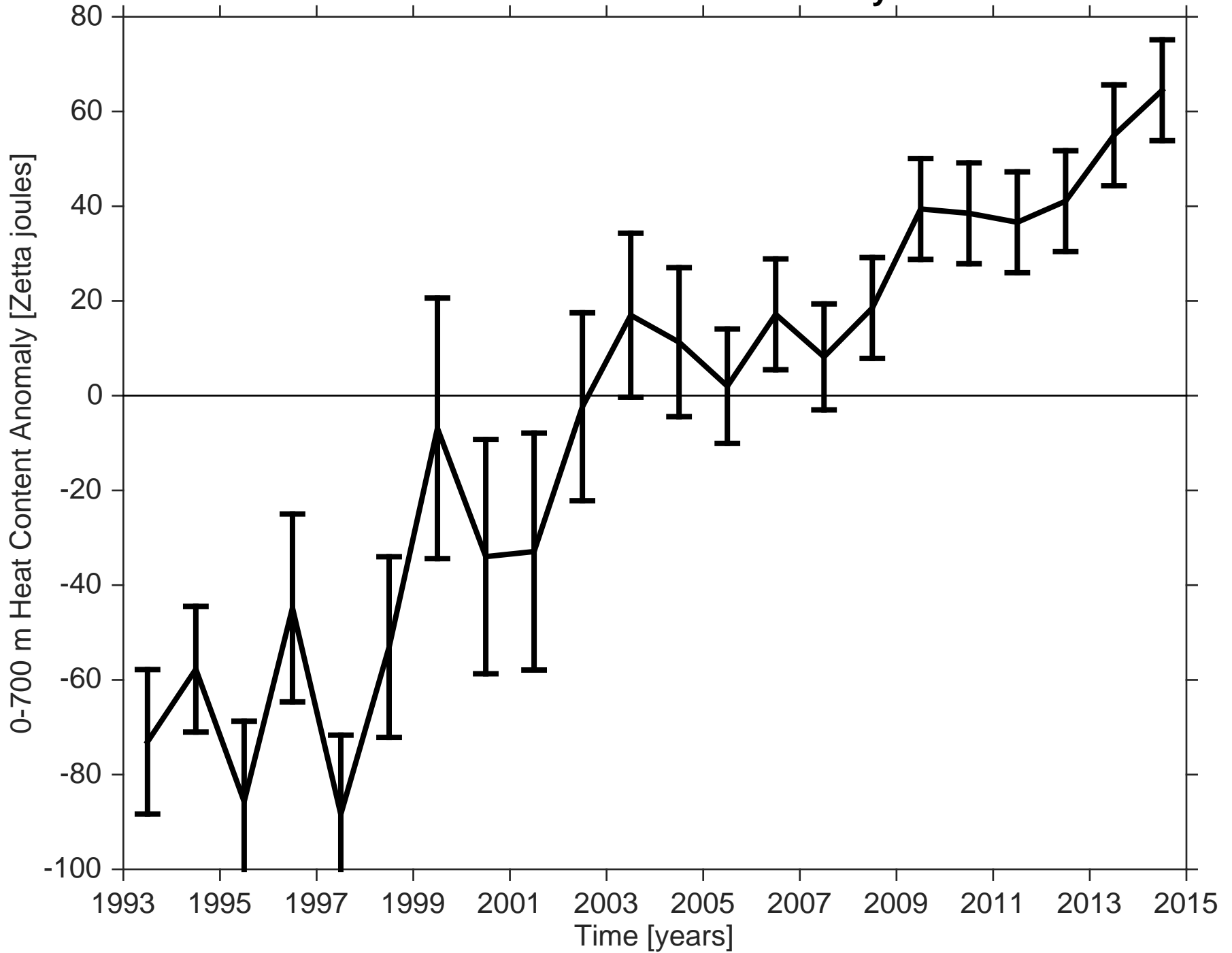
0-700m Heat Content Anomaly
